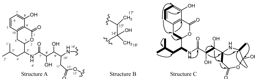
Fig. 2 The selective 2D NMR correlations of 3 . — ^1\text{H} - ^1\text{H} COSY — HMBC.
